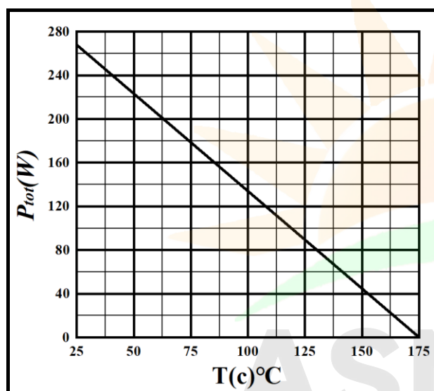
Figure 5. Power Derating
