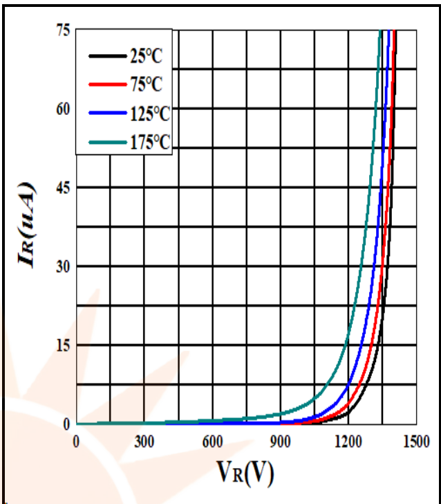
Figure 2. Reverse characteristics
