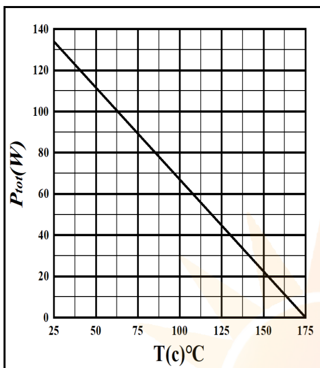
Figure 5. Power derating
