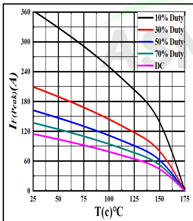
Figure 3. Current derating
